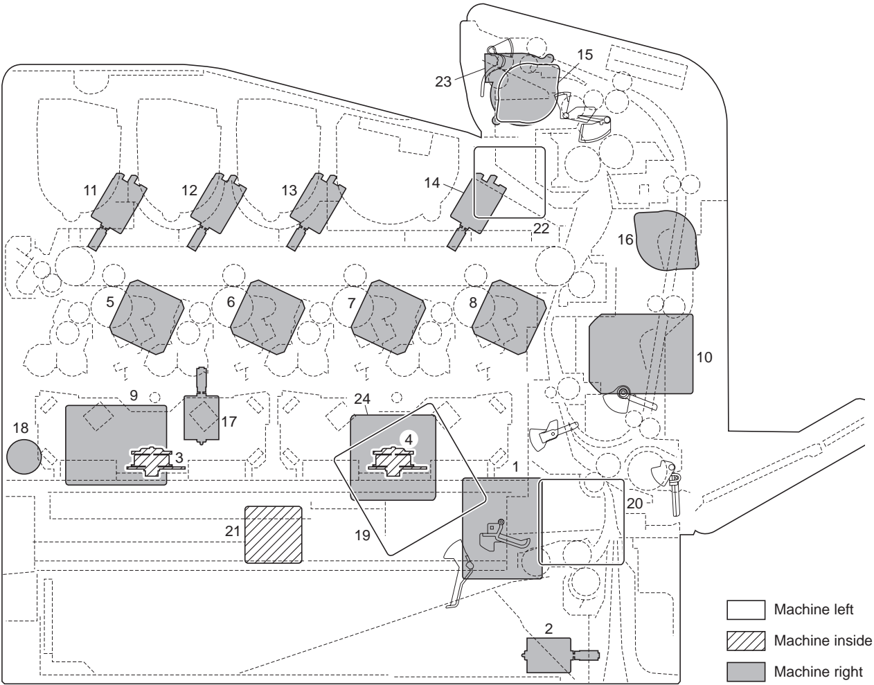
Figure 2-2-3 Motors
