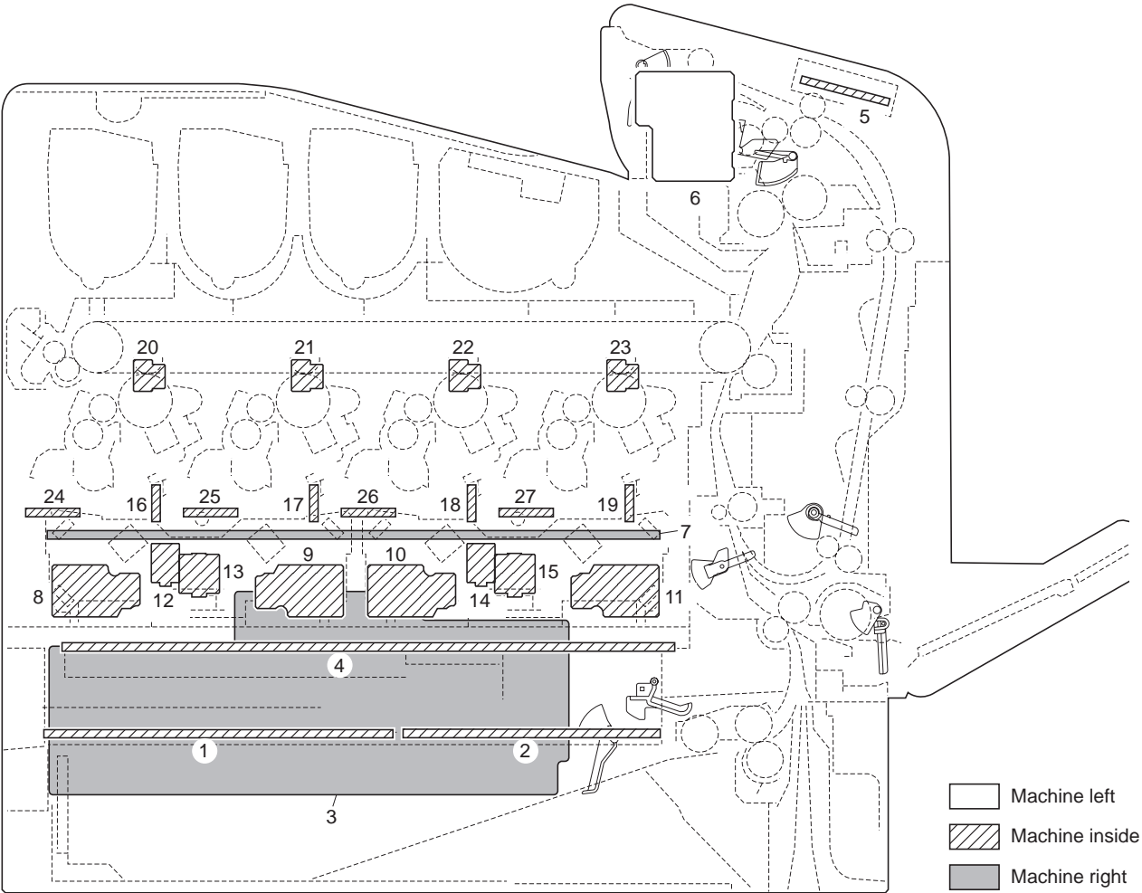
Figure 2-2-1 PWBs
