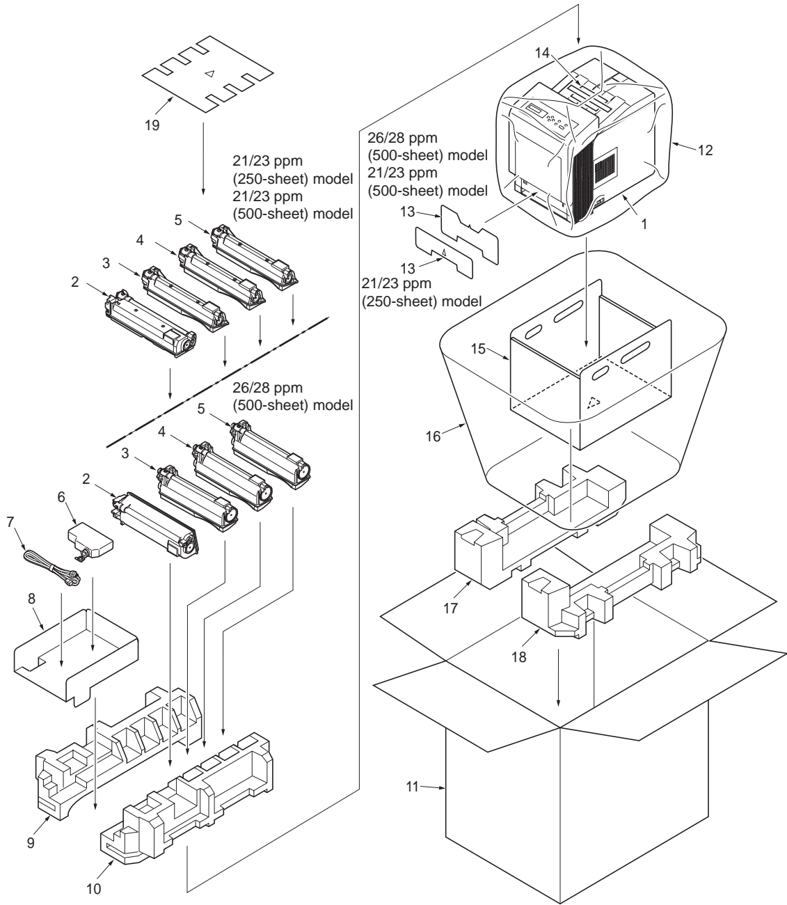
Figure 1-2-3 120 V AC model
