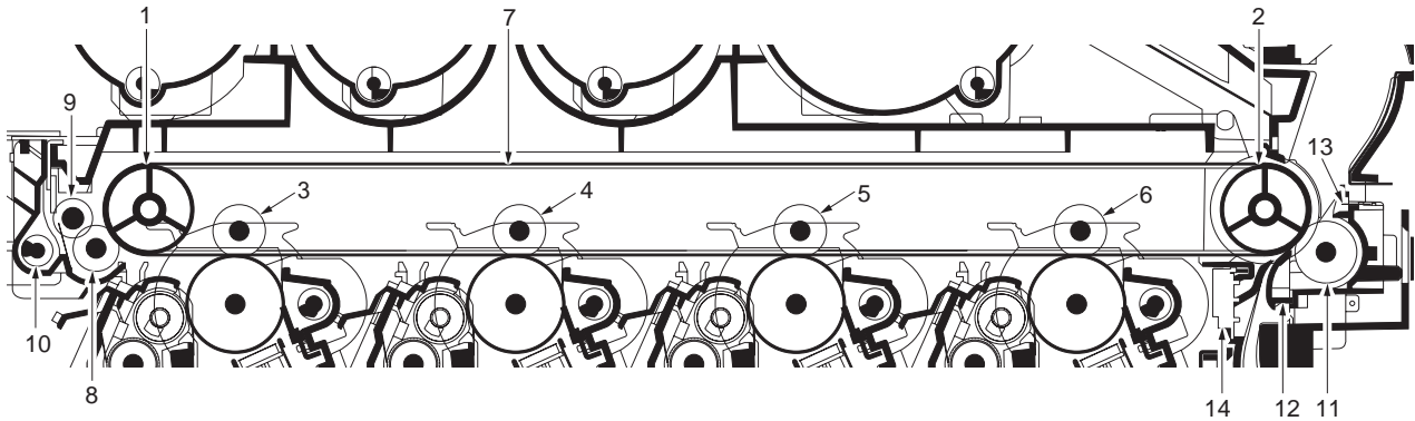
Figure 2-1-16 Transfer/separation section
