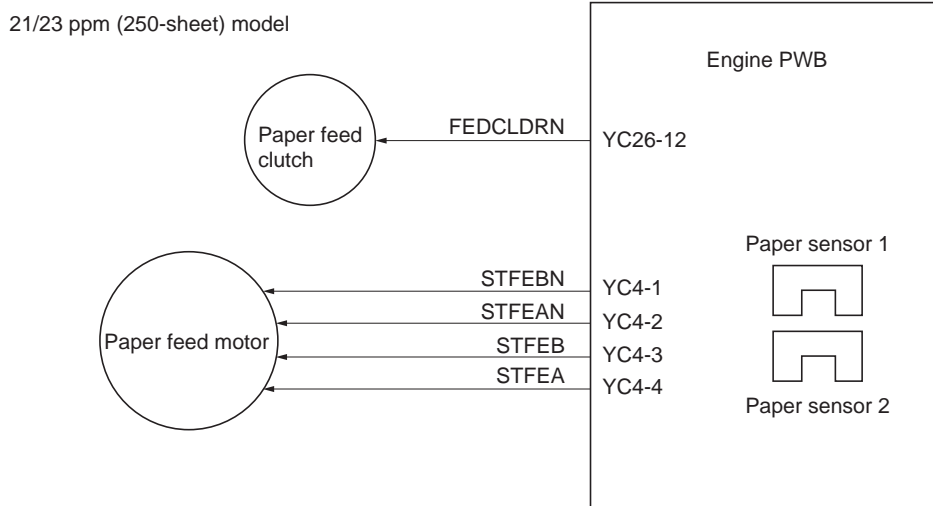
Figure 2-1-2Cassette paper feed section block diagram
